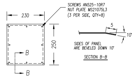
2 BATTERY ACCESS DOOR t=.025" (1 REQ'D)
