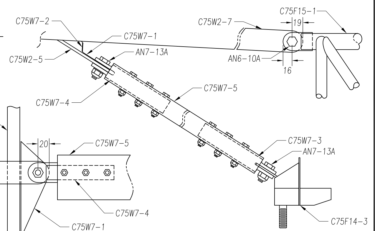
Main Spar and Sturt Attachment
