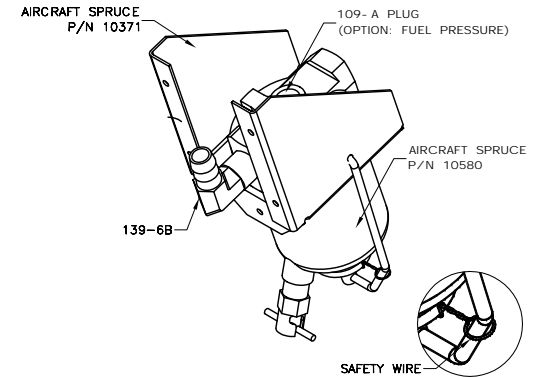
A10580 FUEL GASCOLATOR ASSEMBLY QTY. = 1
