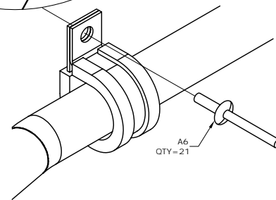
MS2191-DG12 ADEL PADDED CLAMP QTY. = 21
