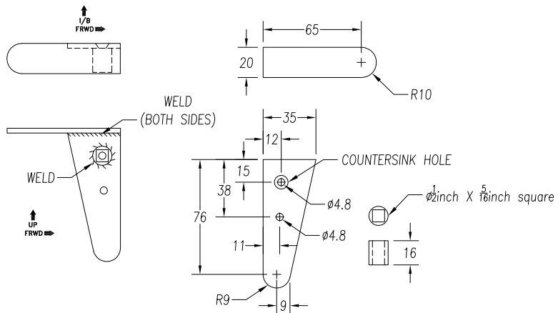
1 0 INTERIOR DOOR HANDLE t=0.125inch 4130 (1L + 1R)
