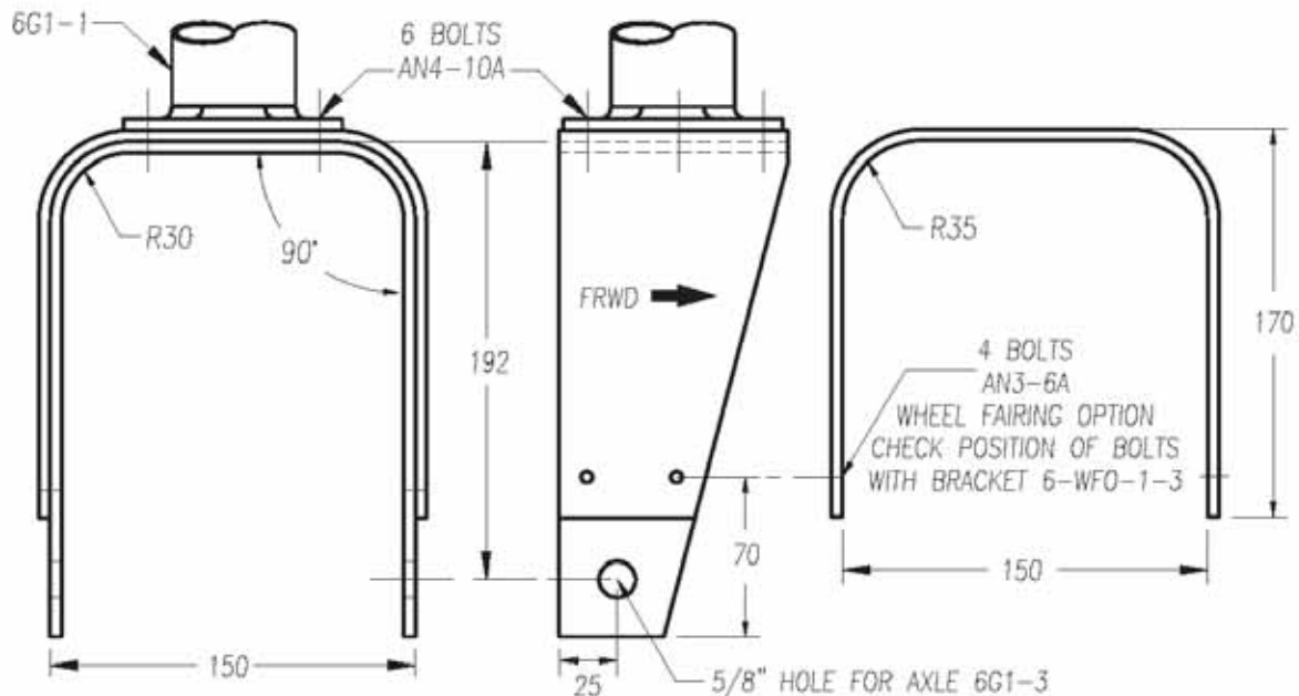
6G1-5 FORK DOUBLER t=3/16" 6061-T6 (1 REQ'D) COLD BEND
